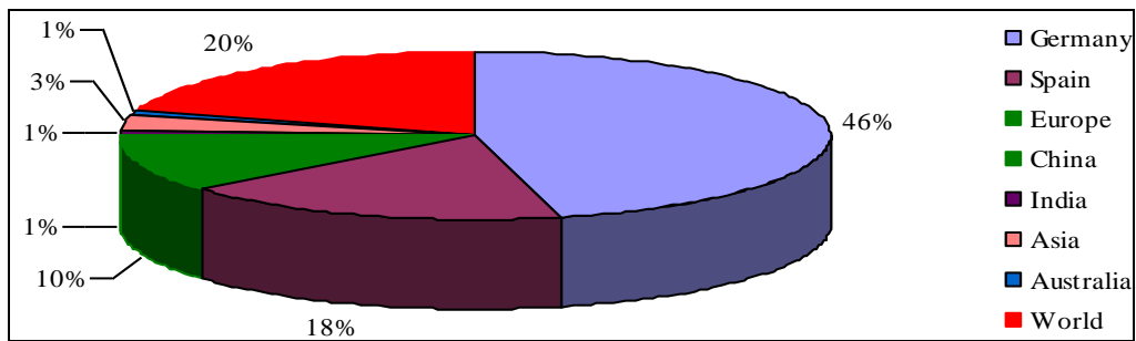
Figure 8. Wind distributions over the world
