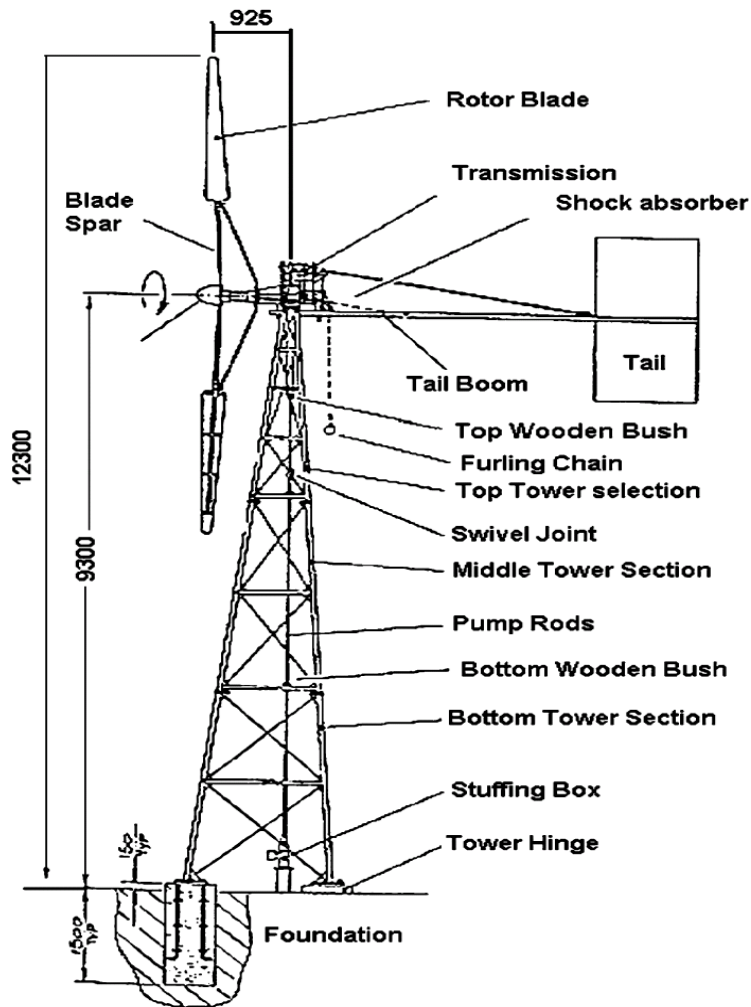
Figure 3. Schematic of the construction of the wind pump.
